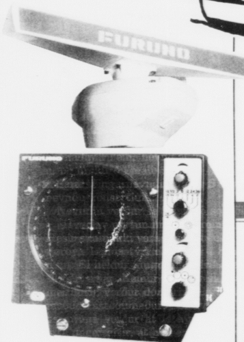
Model FR-240 MK III/ FR-360 MK II 1/4-1/2-1 1/2-3-6-12-24 + 36 sømil (FR 360 MK II) 3 kW sendereffekt 7" PPI/12" linse 3 1/2' antenne
