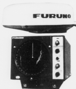
Model 2400 1/4-1/2-2-4-6-12-24 sømil 3 kW sendereffekt 7" PPI/12" linse 3' radomeantenne
