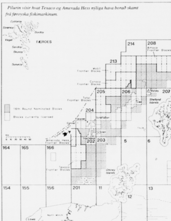
Paleocene oil discoveries
