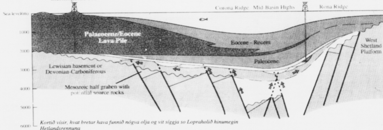
Lopra-1 Traces of thermogenic HC
