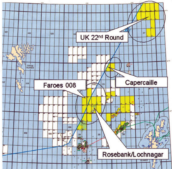
Chevron West of Shetlands Seismic Survey: Acquisition areas
